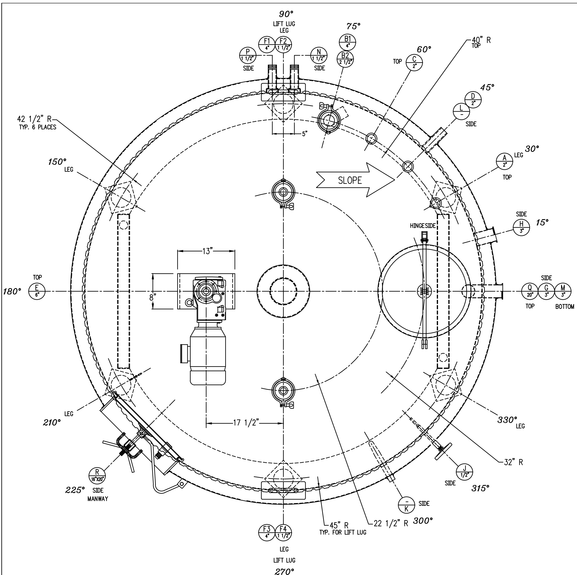
PLAN VIEW HBT1 (TK-3390)
